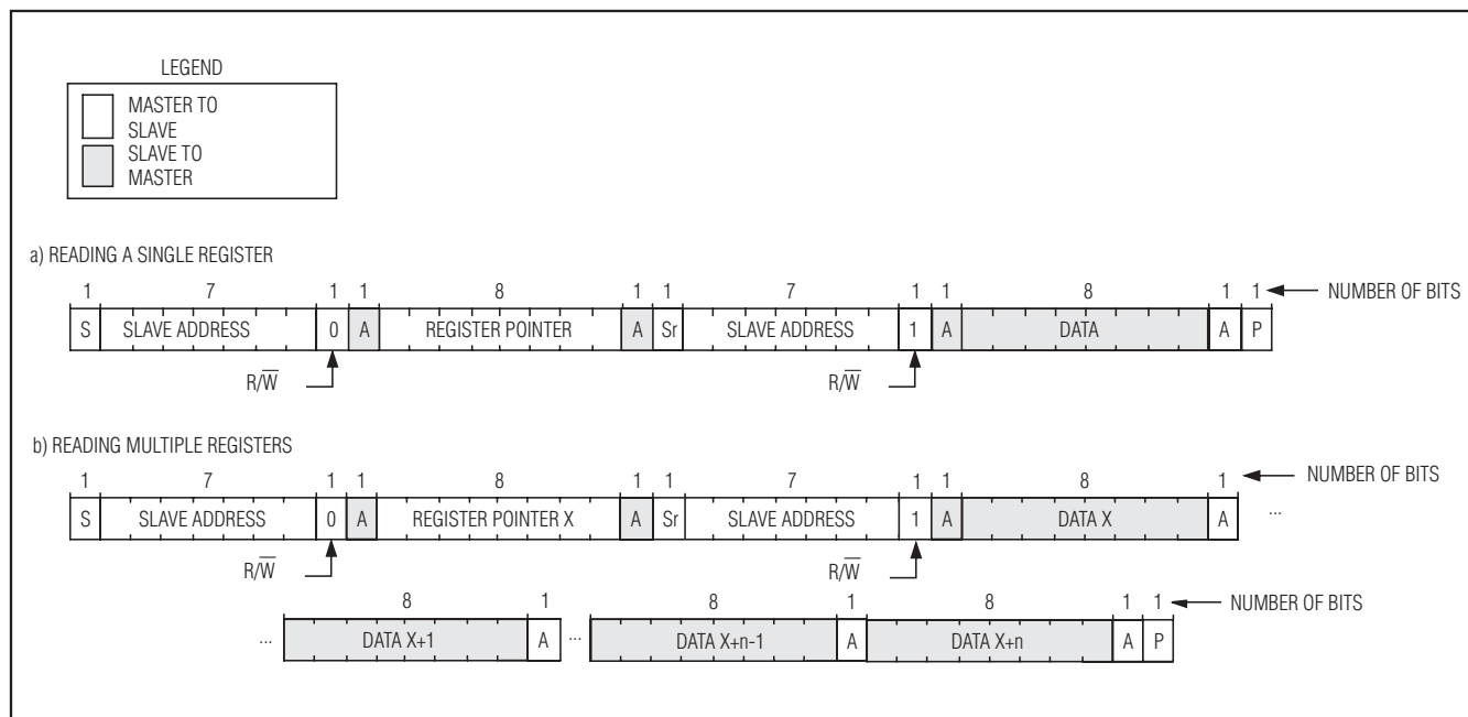
Figures 15a and 15b. Reading from the ICs
